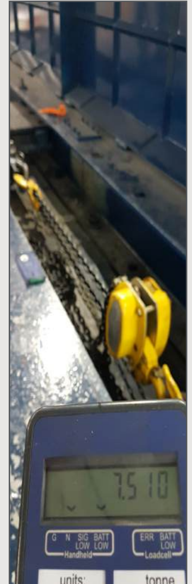
PROOF LOAD TEST OF CHAIN BLOCK
