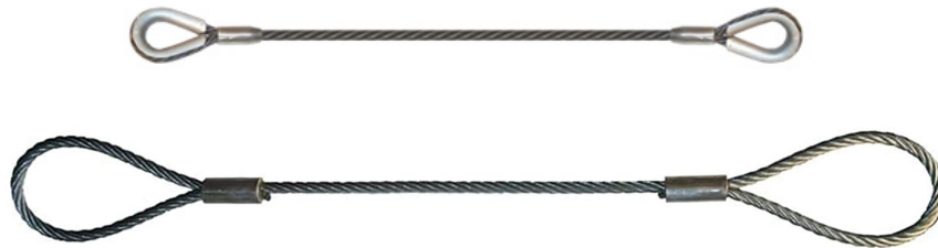
IWRC Construction - 1960 Grade - Class 6x19, Class 6x36
